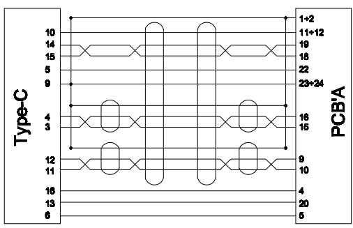
PIN OUT
